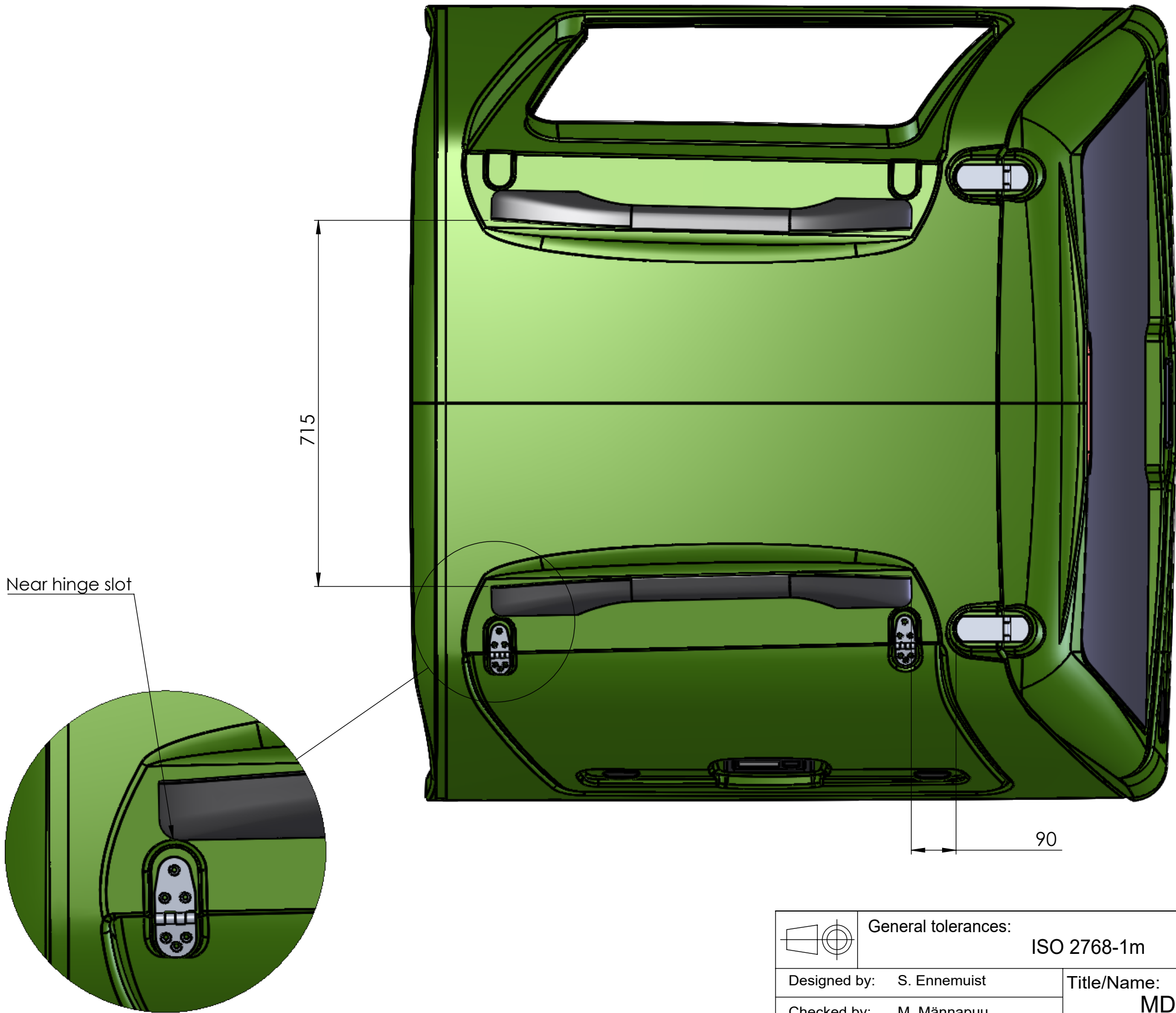
DETAIL A SCALE 1 : 4
